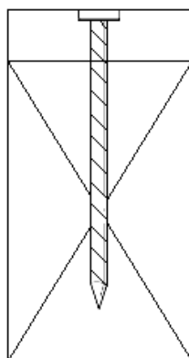
Side Member
